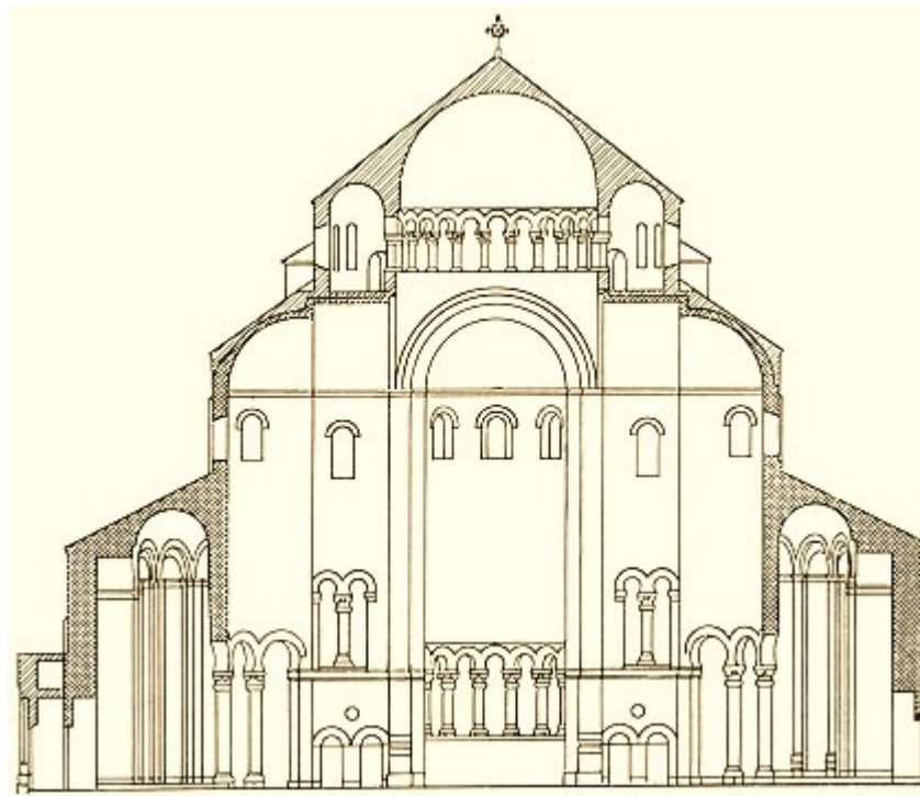
The Zvartnots Cathedral. A two-dimensional [internal - external ] view.
