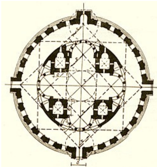
The crisscrossing grids forming a harmonious symmetry. General layout of the Zvartnots-esque Banak Cathedral in the Tayk' Province of Armenia.
